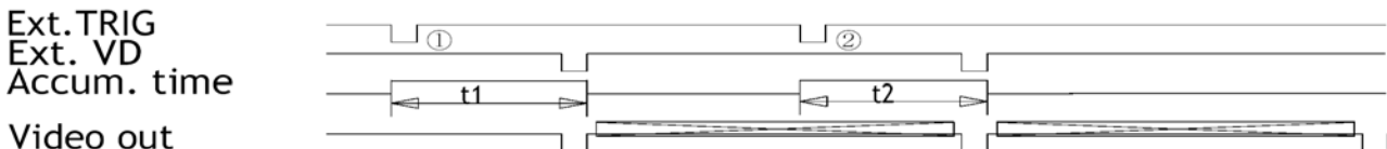
Fig. 25. Start stop non-interlaced field integration
