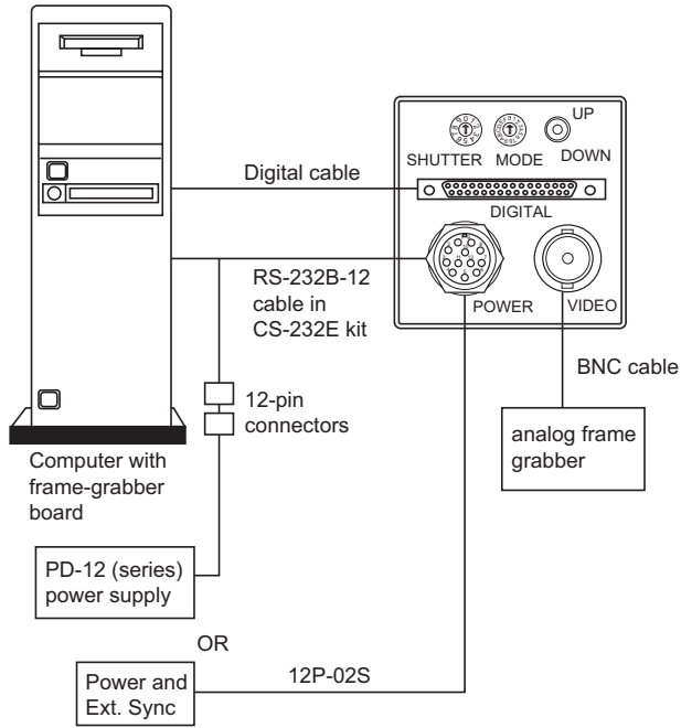
FIGURE 2. TM-1402CL System Configuration
