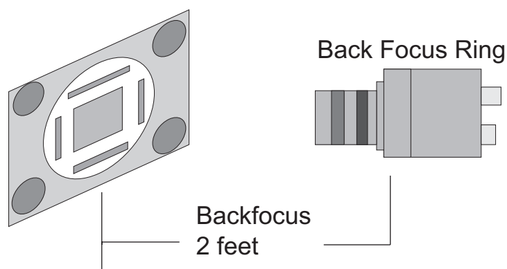
FIGURE 8. Back Focus Adjustment
