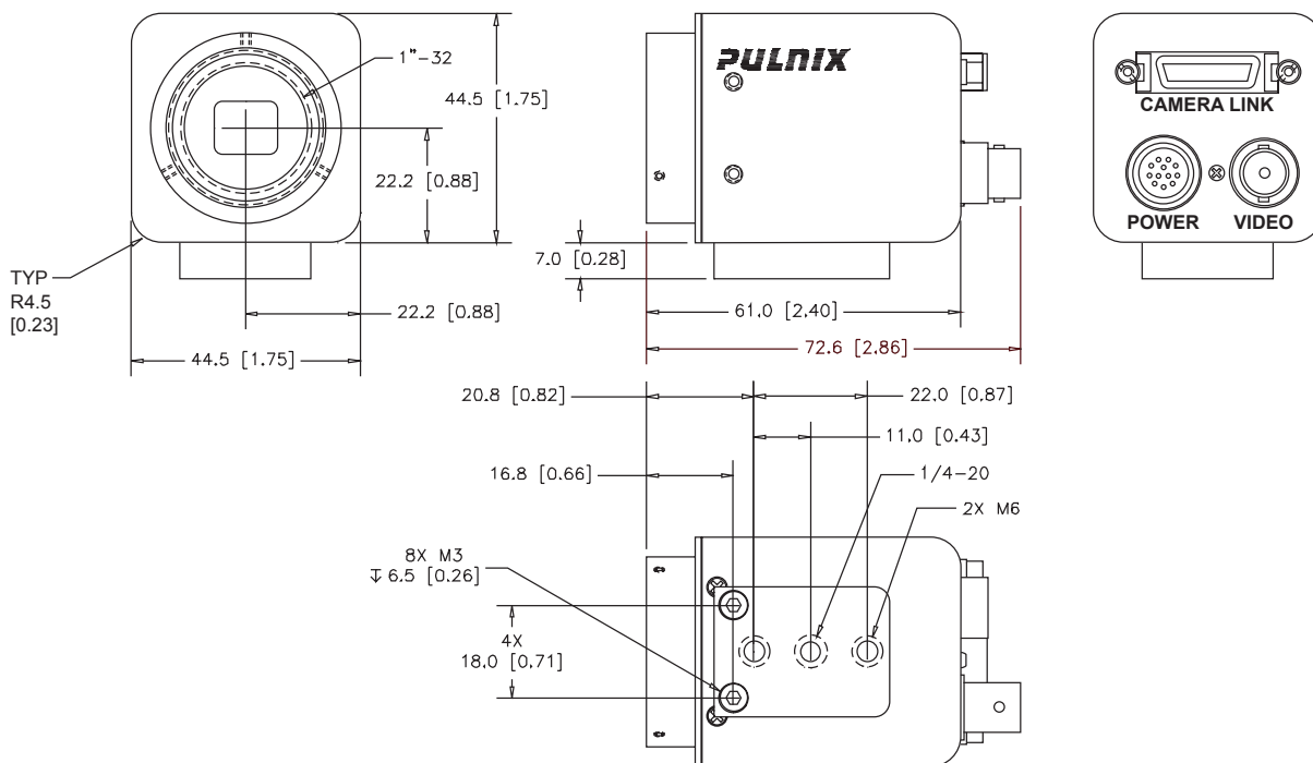
FIGURE 11. Physical Dimensions (TM-1402CL)
