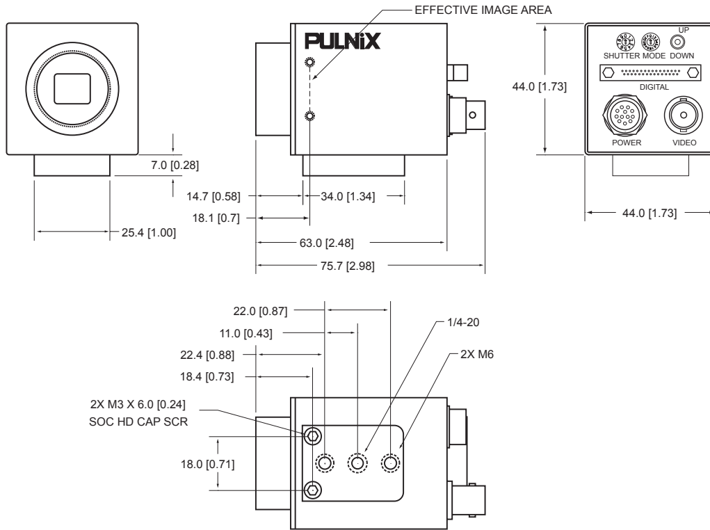
FIGURE 11. Physical Dimensions (TM-1402CL)
