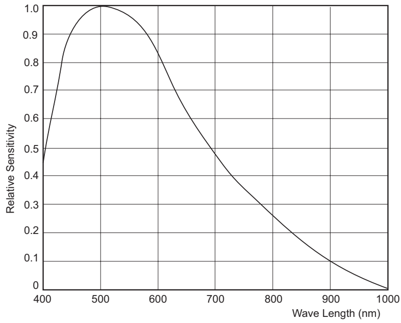
FIGURE 12. Spectral Response
