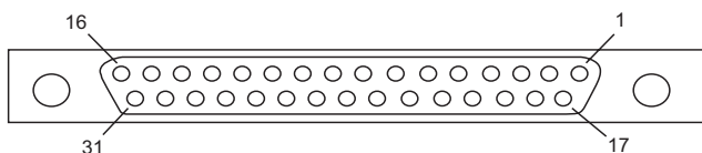
FIGURE 4. 31-Pin Digital Connector on Rear Panel of Camera (TM-1402 only)
