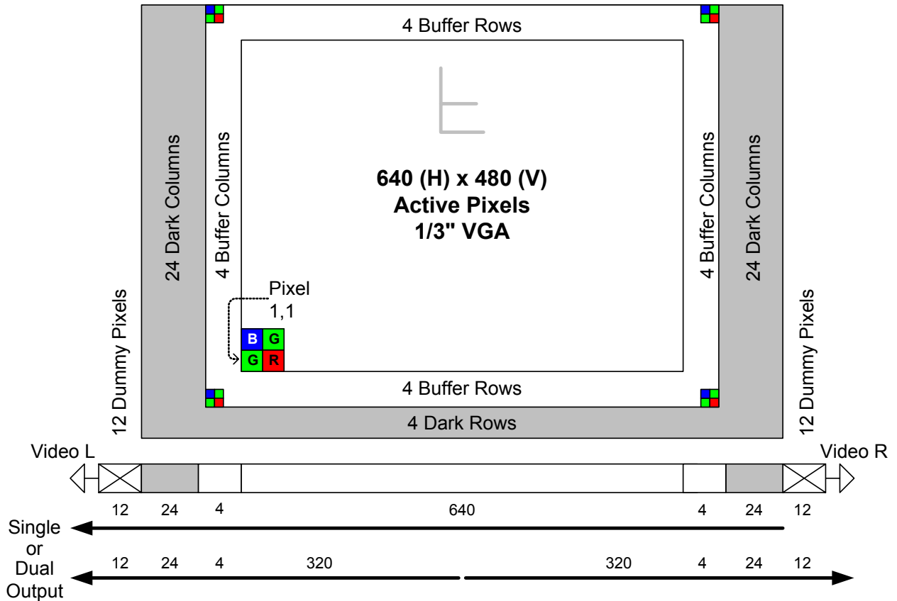
Figure 1 - Sensor Architecture
