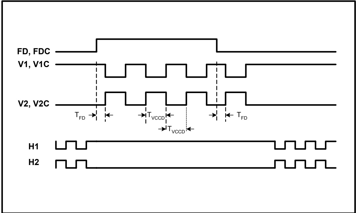
Figure 14 - Fast Line Dump Timing
