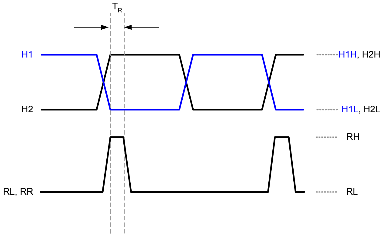
Figure 11 - Pixel Timing Detail
