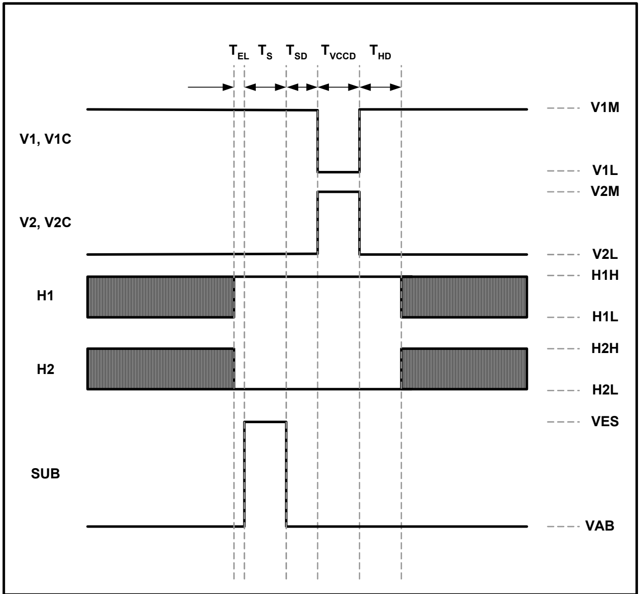
Figure 12 - Electronic Shutter Timing
