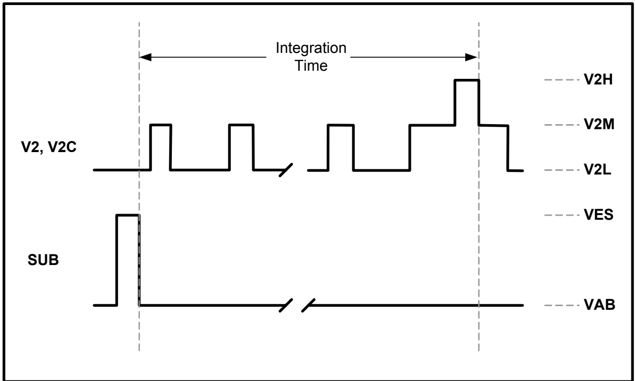
Figure 13 - Integration Time Definition
