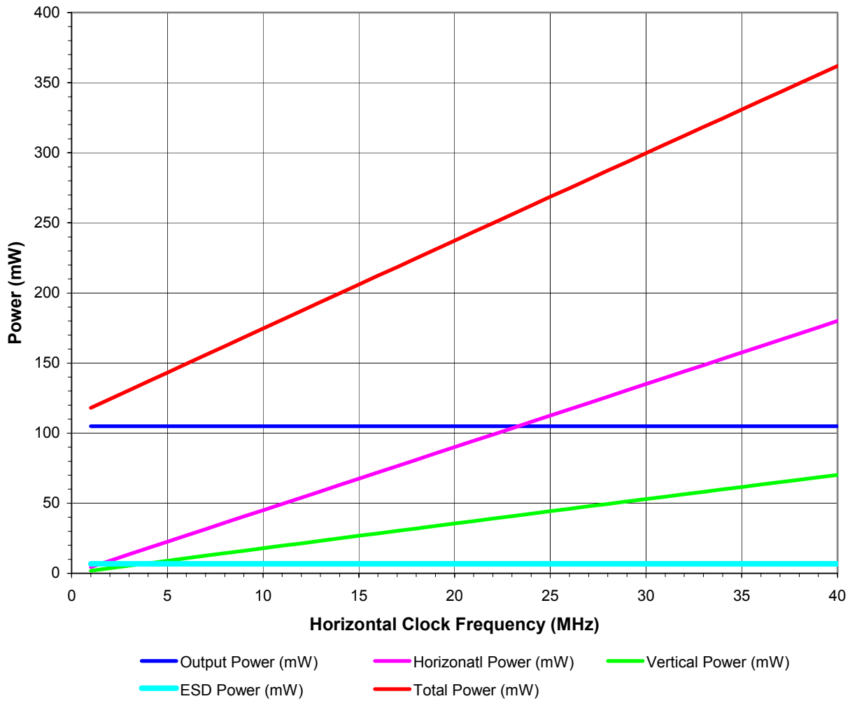
Figure 3 - Power
