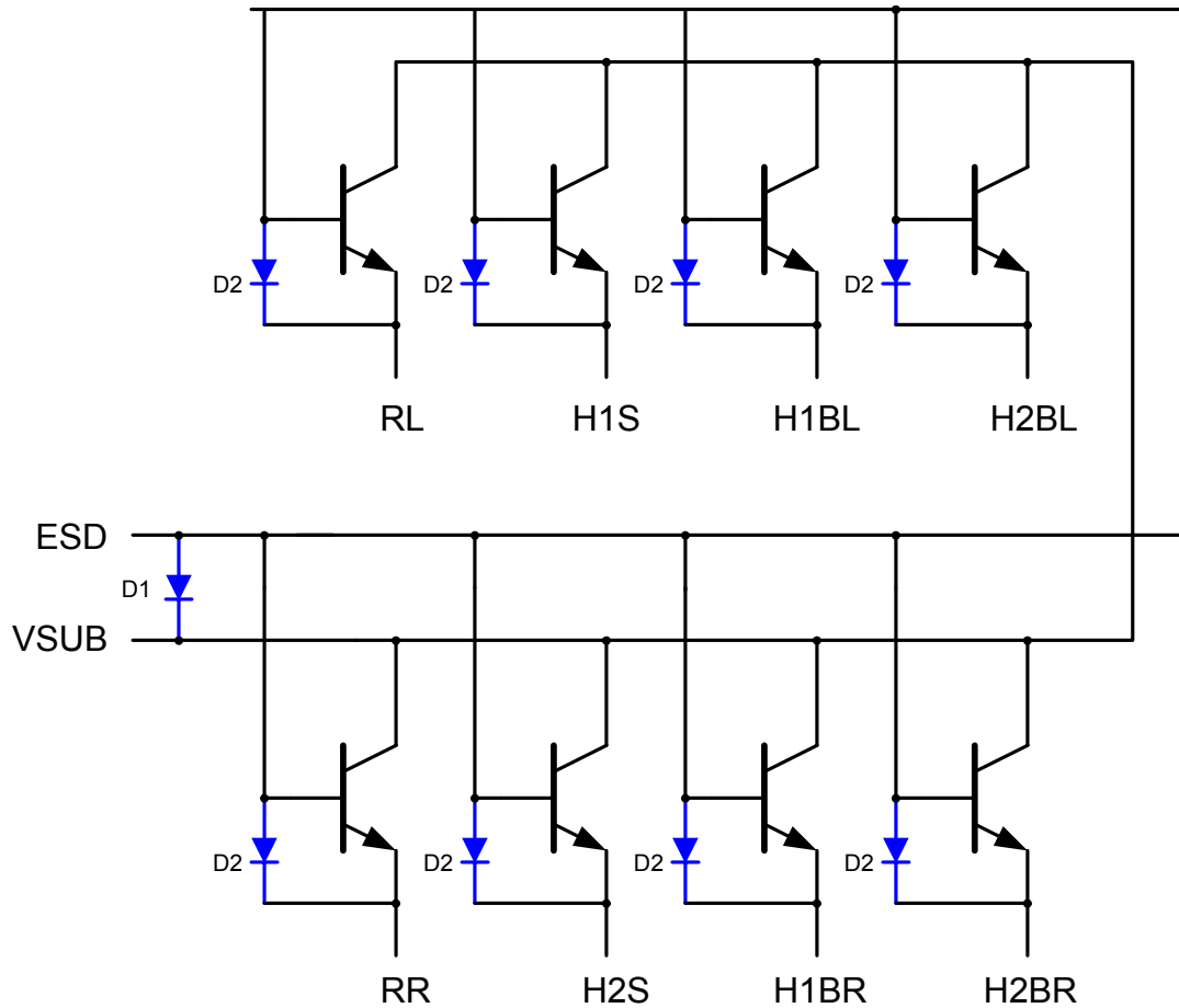
Figure 2 - ESD Protection
